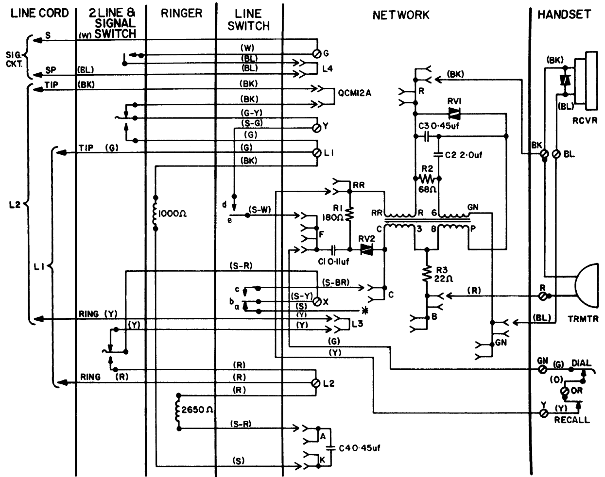
Schematic Diagram – QSK110A Telephone Set (For Sets equipped with QNB425E1A Network)
