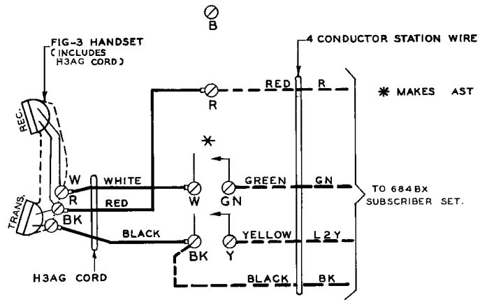
No. 211A-3 Hand Telephone Set for Anti-Sidetone, Manual Common Battery Service
