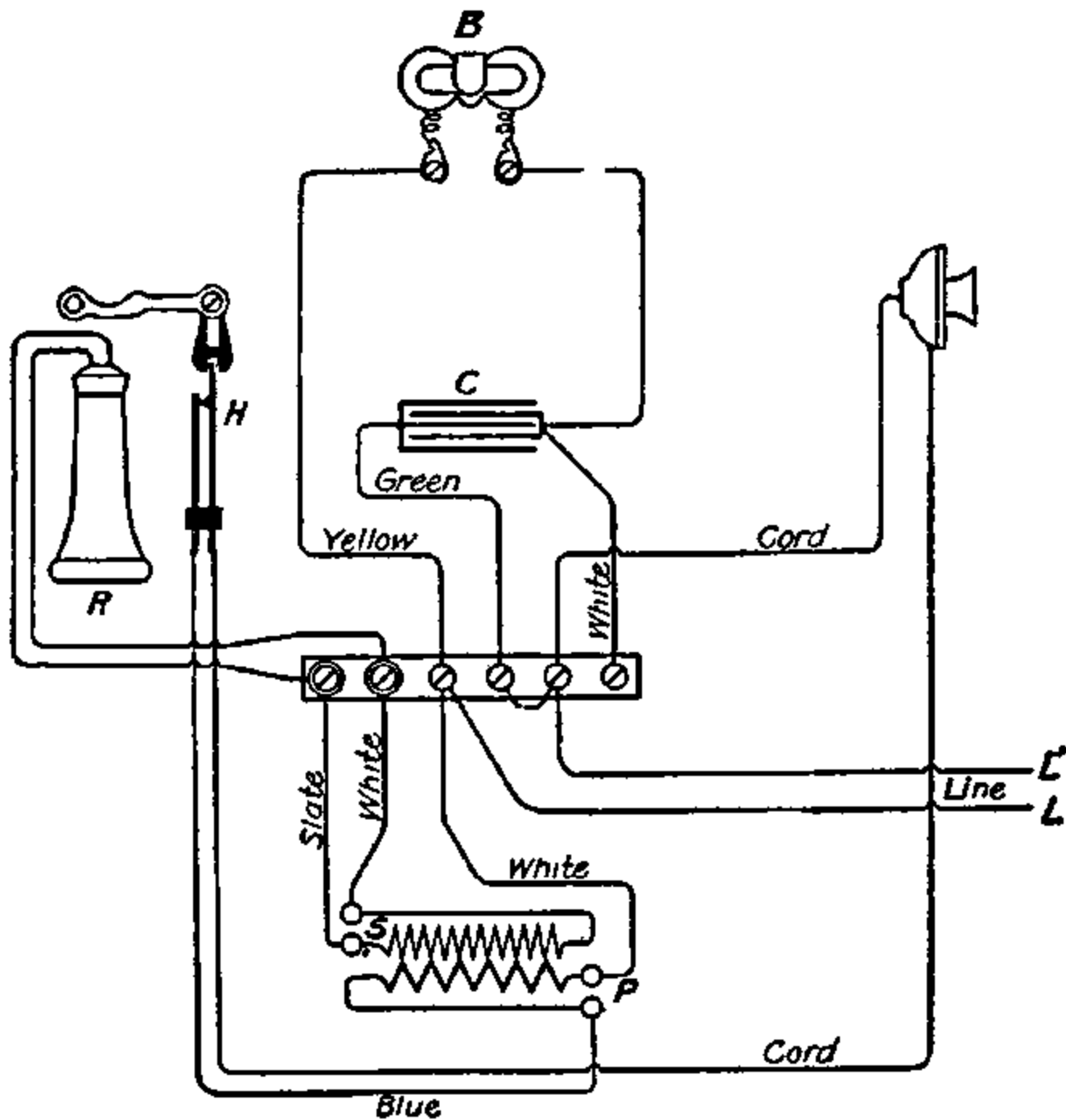
CIRCUITS OF NORTH ELECTRIC CO. COMMON BATTERY WALL TELEPHONE
