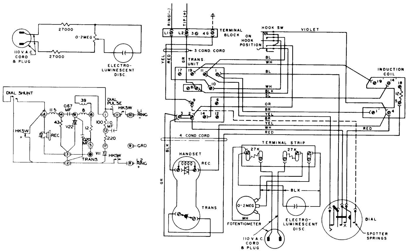
Schematic and wiring diagram for Type 182 telephone.
