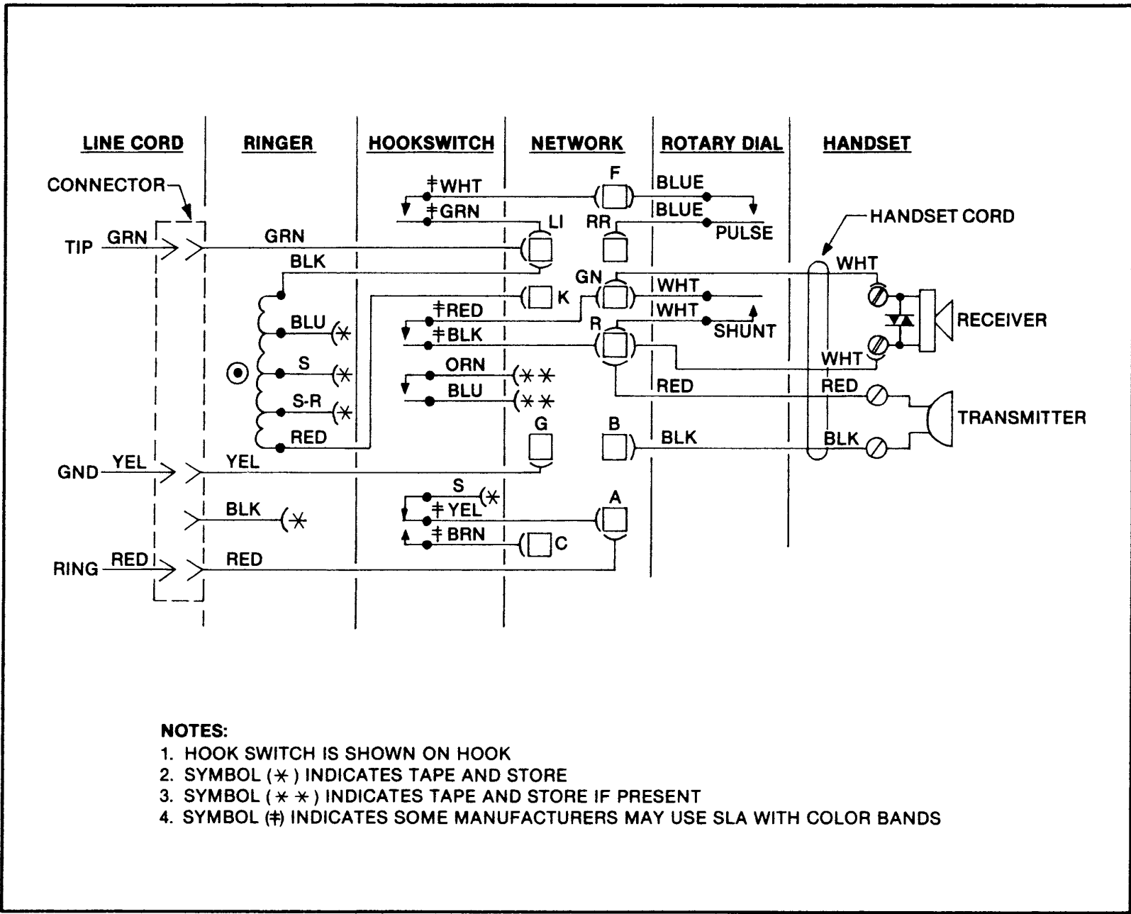
Rotary Dial Wiring Diagram
