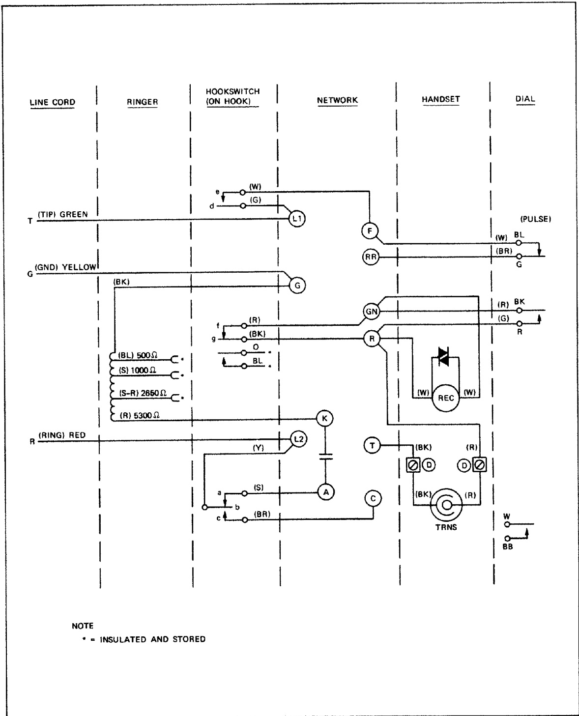
BS-4100 Series Wiring Diagram Using SC 703013-416 Network
