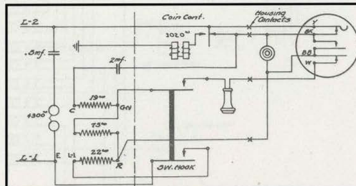
150 H & HJ PREPAYMENT PAYSTATION WITH 684-BA3 DESK SET BOX Equipped With Dial Shorting Springs
