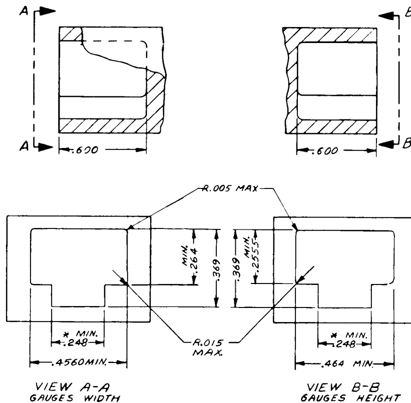
NO - GO GAUGE
