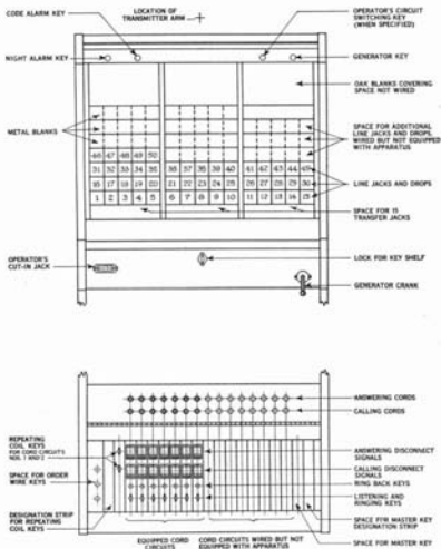
Fig. 24—Standard Equipment of No. 105-B Magneto Switchboard.
