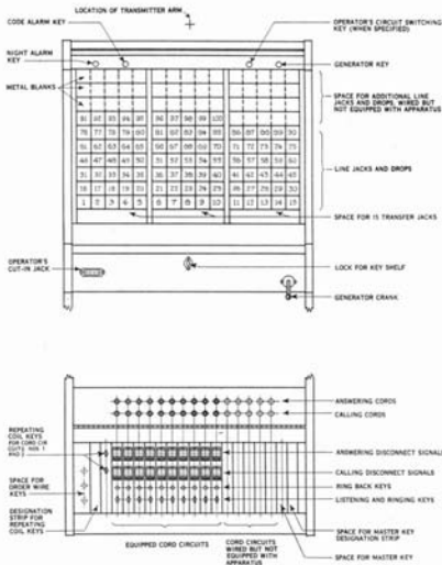
Fig. 25—Standard Equipment of No. 105-C Magneto Switchboard.
