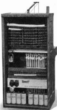
Fig. 4—Rear View No. 105-C High Efficiency Switchboard
