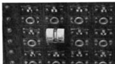
Fig. 10—Appearance of No. 11 Type Drop shutter when viewed from above.
