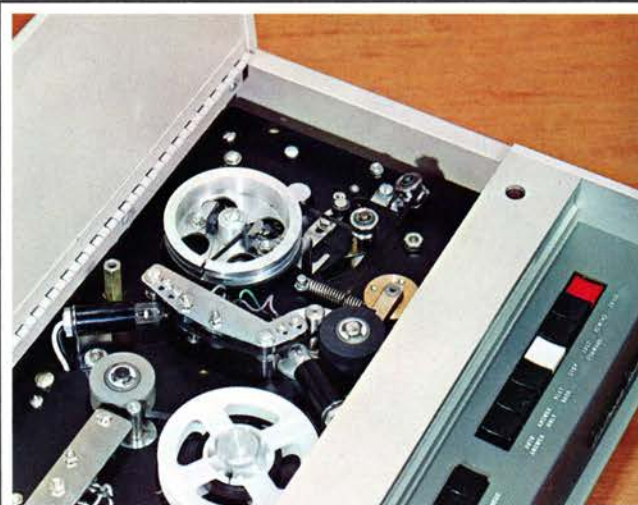
ANNOUNCEMENT LENGTH CAN BE VARIED BY SUBSCRIBER from five seconds to three minutes. Machine resets itself to receive calls immediately after announcement, whether announcement is long or short. Each new announcement completely erases the one preceding it.
