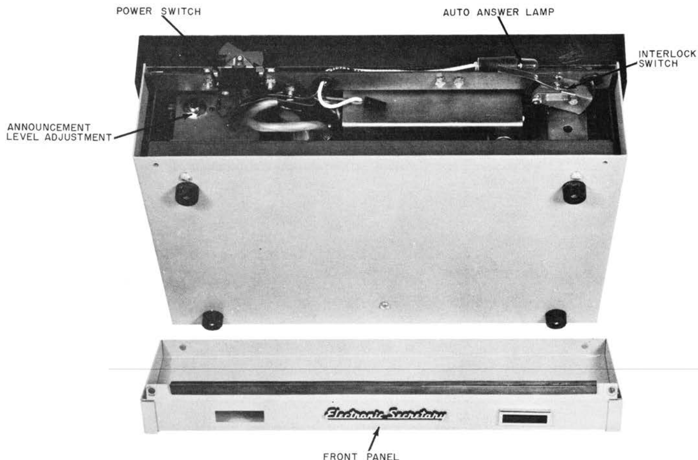
Figure 4. AO-3 with front panel removed.
