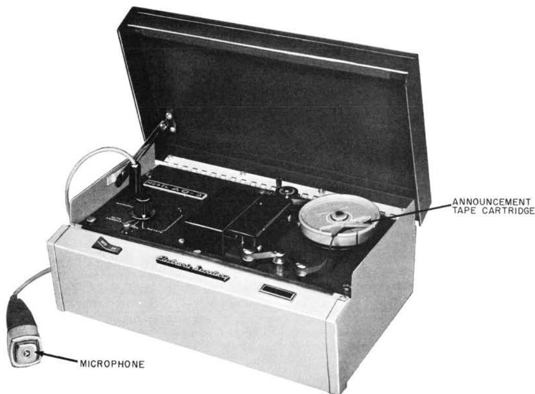
Figure 1. Model AO-3 (front view).
