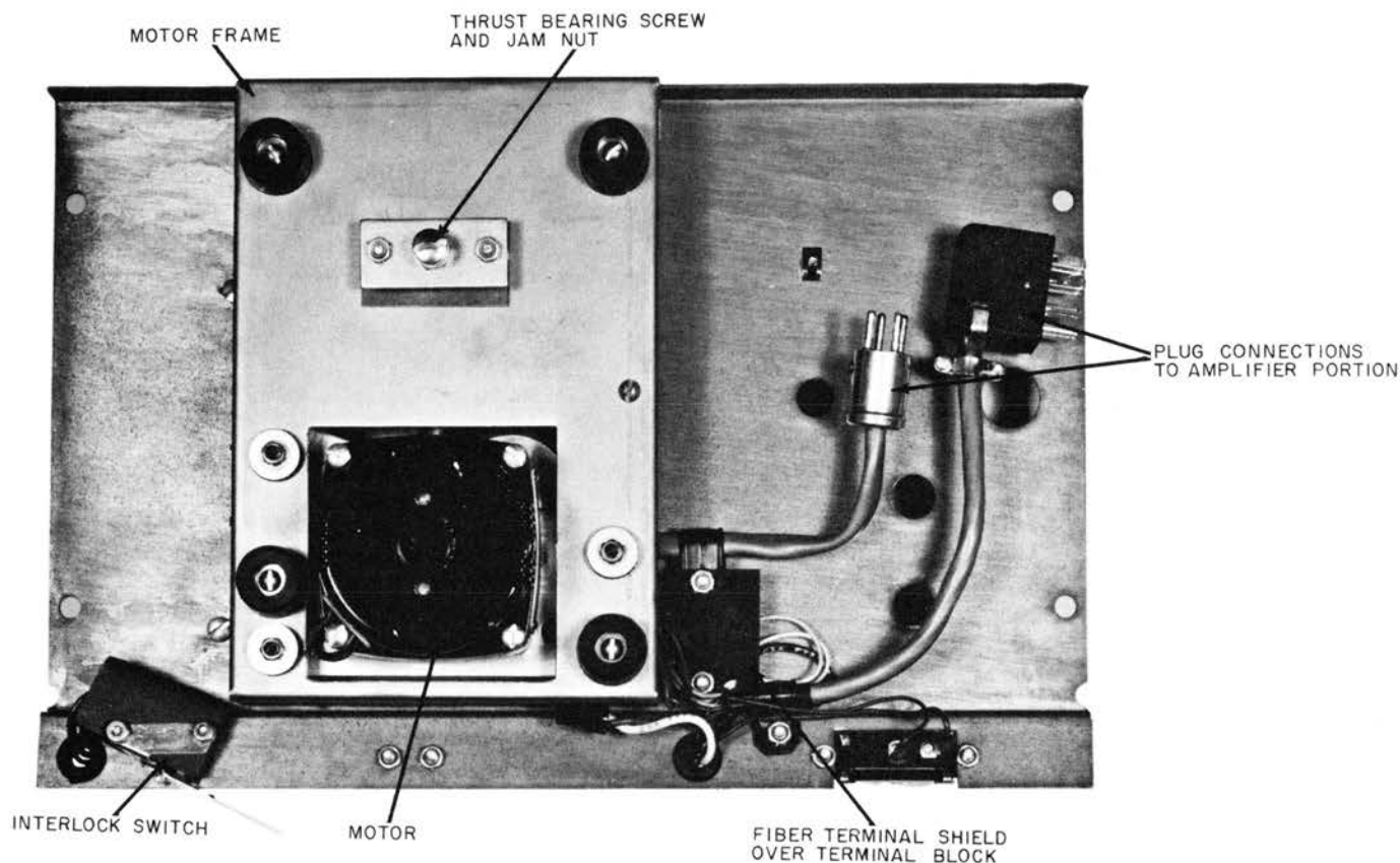
Figure 2. Bottom of tape mechanism.
