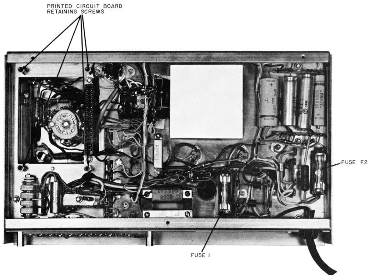
Figure 5. Bottom of amplifier housing.
