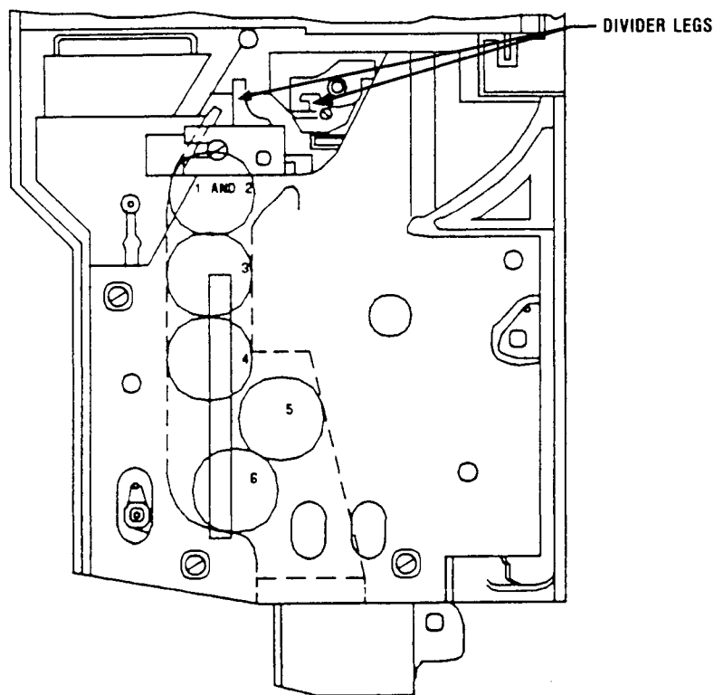
Figure 25 Coin Chute
