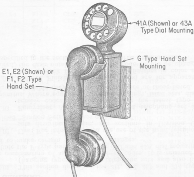
Fig. 1—Typical 211, 212, 213 and 214 Hand Telephone Sets
