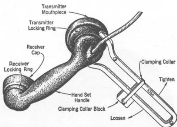
Fig. 3—Correct Positioning of a Single 438A Tool
