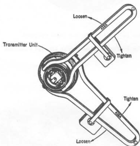
Fig. 4—Correct Positioning of Two 438A Tools
