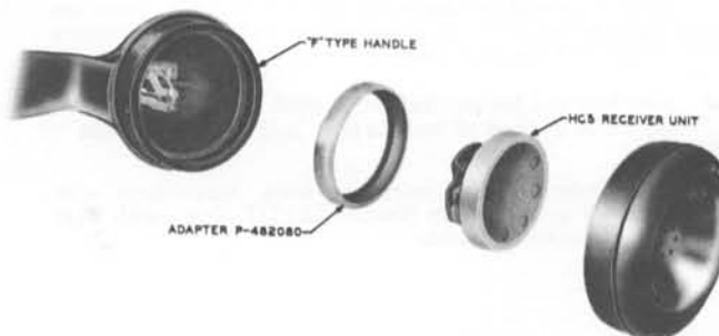
Fig. 8—HC-5 Receiver Unit and Adapter, Order of Assembly
