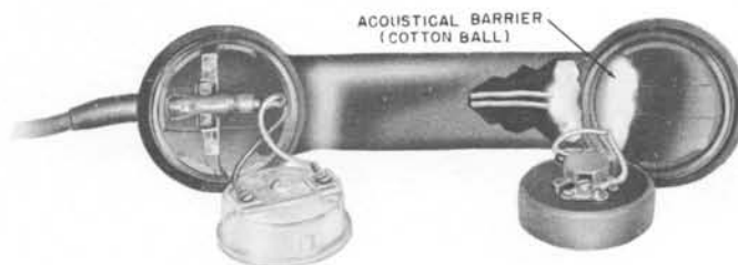
Fig. 9—G3' Handset, Placement of Acoustical Barrier
