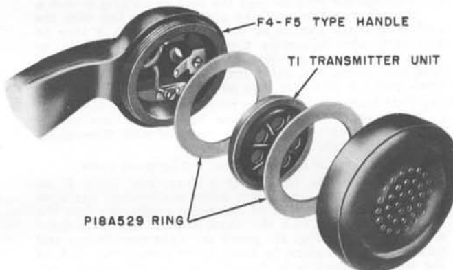
Fig. 7—F4- and F5-type Handset, Order of Assembly of the T1 Transmitter Unit Rings and Cap
