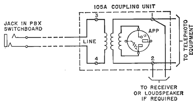
Fig. 6 — Special PBX Extension Connections (No Set Required)
