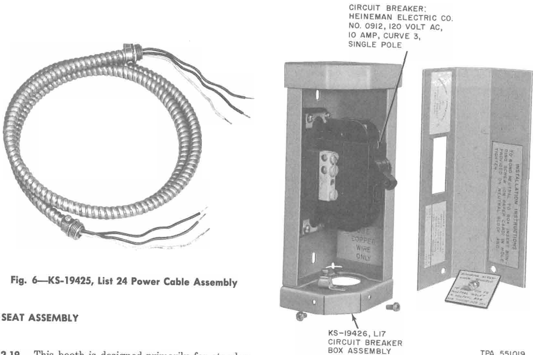
Fig. 7—Circuit Breaker and Box Assembly
