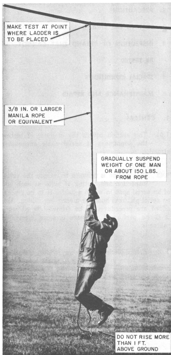
Fig. 1—Testing Strand Prior to Placing Ladder
