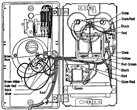
Fig. 3 — 354C Telephone Set with 6 Type Dial
