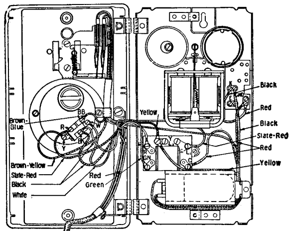
Fig. 5 — 356C Telephone Set with 6 Type Dial
