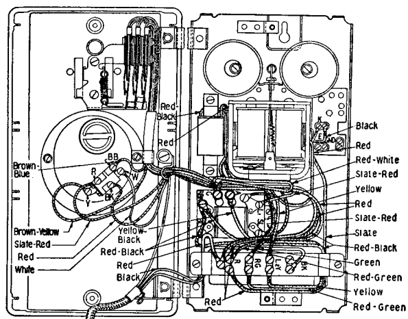
Fig. 7 — 357C Telephone Set with 6 Type Dial
