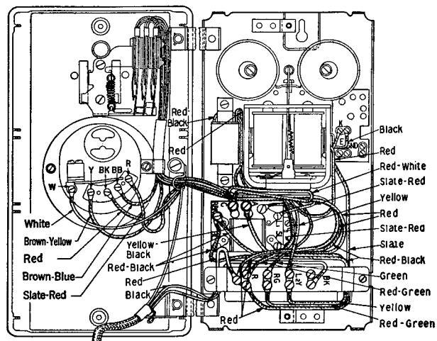
Fig. 6—357C Telephone Set with 4 or 5 Type Twin Contact Dial
