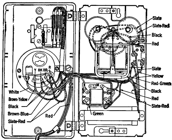
Fig. 2 — 354C Telephone Set with 4 or 5 Type Twin Contact Dial
