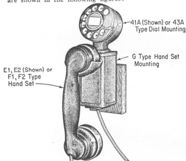
Fig. 1—Typical 211, 212, 213 and 214 Hand Telephone Sets
