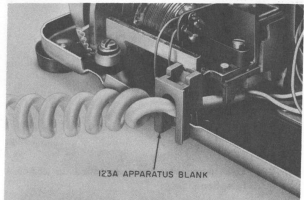
Fig. 32—123A Apparatus Blank Installed on 2500D1M Telephone Set Base
