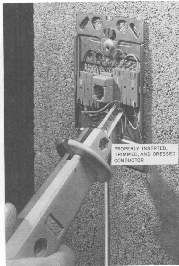
Fig. 14—Connecting Wire With Lead Insertion Tool
