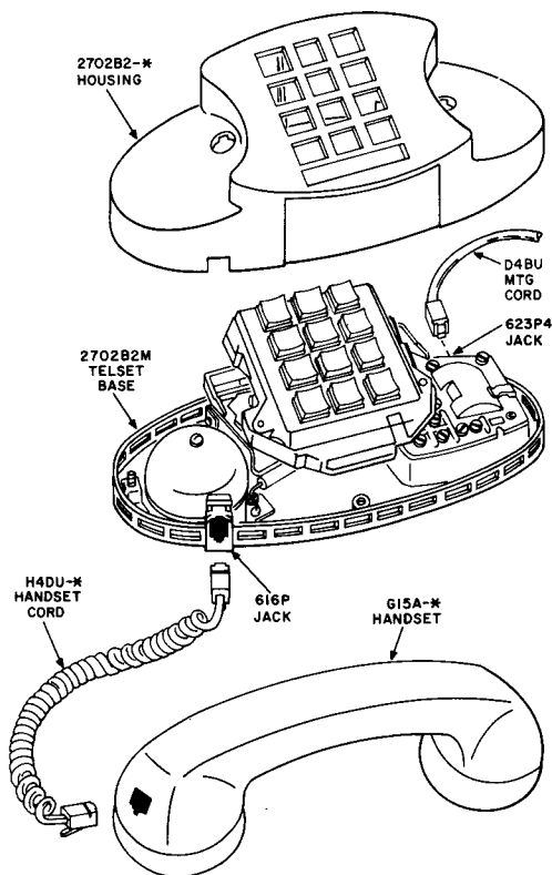
2702BM TELEPHONE SET
