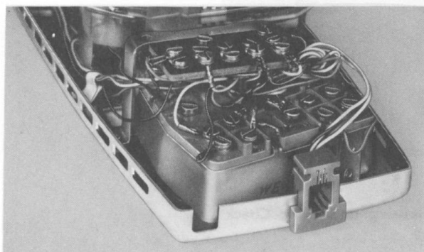
Fig. 45—2554B2M Telephone Set Base With Handset Cord Jack Installed
