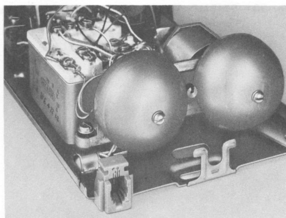
Fig. 36—554B2P Telephone Set Base With Handset Cord Jack Installed
