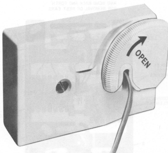
Fig. 9—625S Connecting Block With D4BU Cord Inserted.
