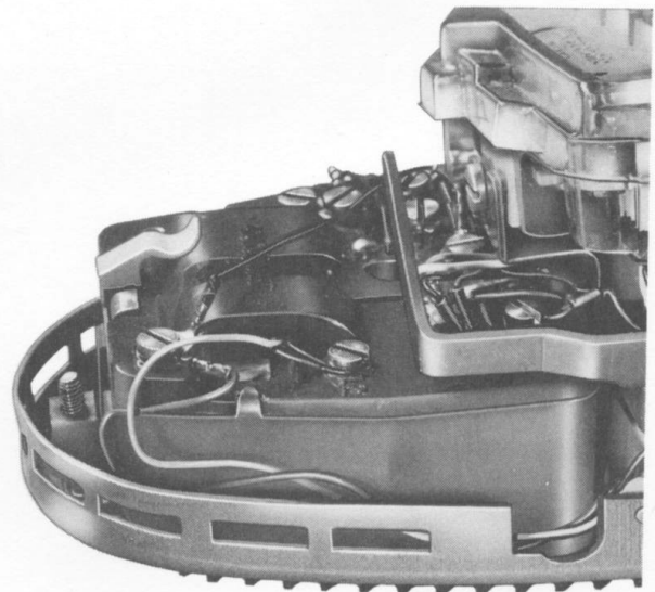
Fig. 40—PRINCESS Telephone Set Base Modified to Accommodate Mounting Cord Jack
