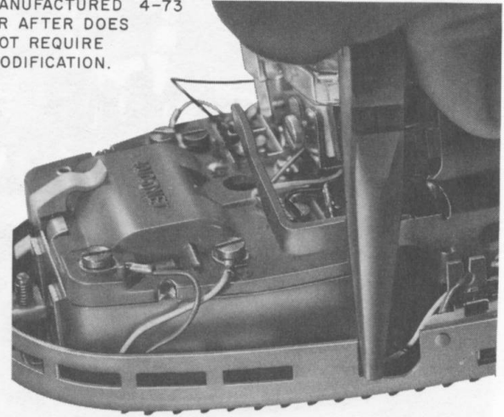
Fig. 39—Modifying PRINCESS Telephone Set Base to Accommodate Mounting Cord Jack
