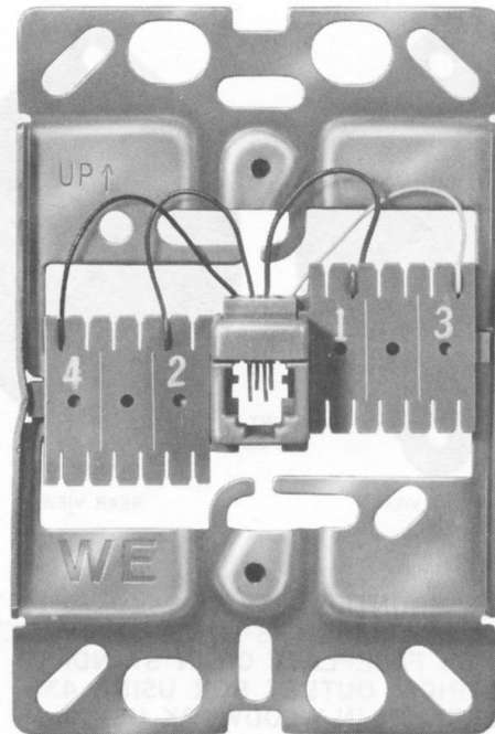
Fig. 12—630A4 Connecting Block With Newer Bracket - Refer to Fig. 11 For Mounting Instructions
