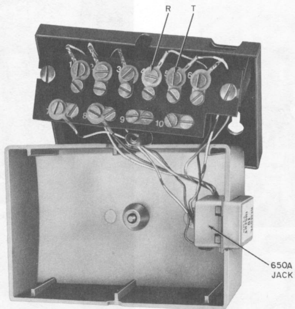
Fig. 15—635A Connecting Block
