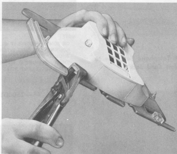
Fig. 48—Notching 2702B1 Housing and Using Check Gauge
