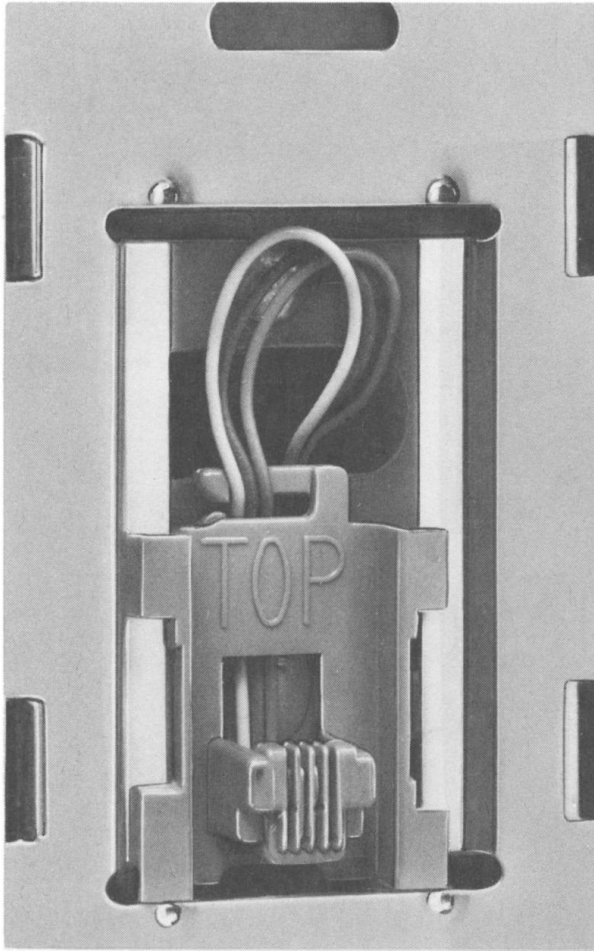
Fig. 23—Partial View of 228-Type Adapter With 523A3 Plug, Showing Slack Loop in Plug Leads
