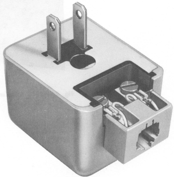
Fig. 25—248A Adapter as Used With 2012 Transformer
