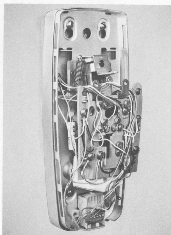
Fig. 35—AC1MP Telephone Base
