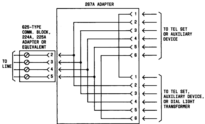
Fig. 27—Schematic of 267A Adapter
