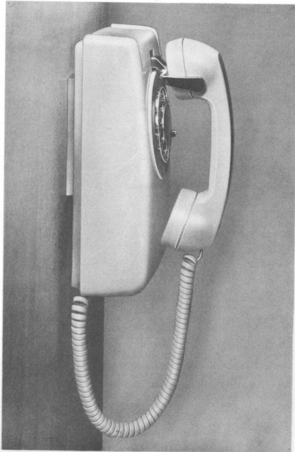
Fig. 30—554BMP Telephone Set on 630A-Type Connecting Block
