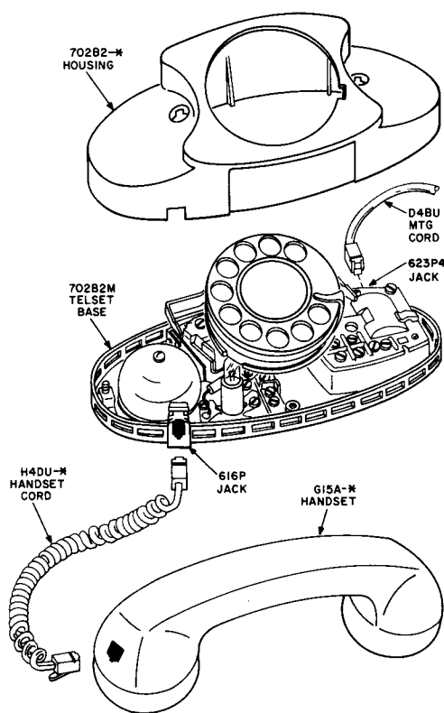
702BM TELEPHONE SET
