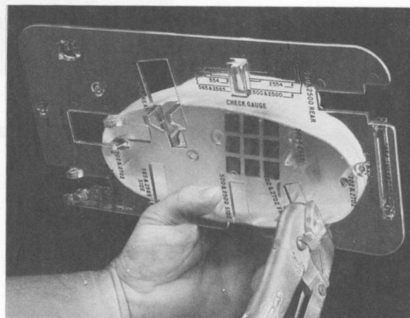
Fig. 47—Positioning Notching Tool (2702B1 Housing on Template)
