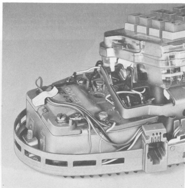
Fig. 41—PRINCESS Telephone Set Base With Mounting Cord Jack Installed
