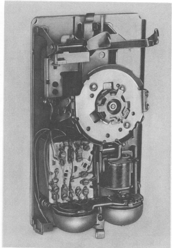
Fig. 31—554B2P Telephone Set Base
