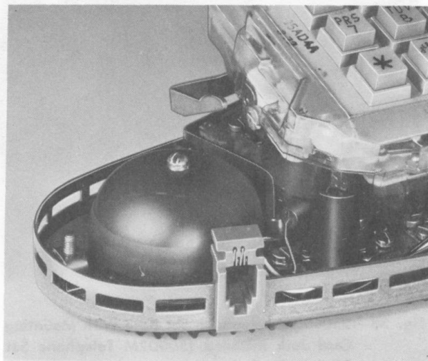
Fig. 43—PRINCESS Telephone Set Base With Handset Cord Jack Installed
