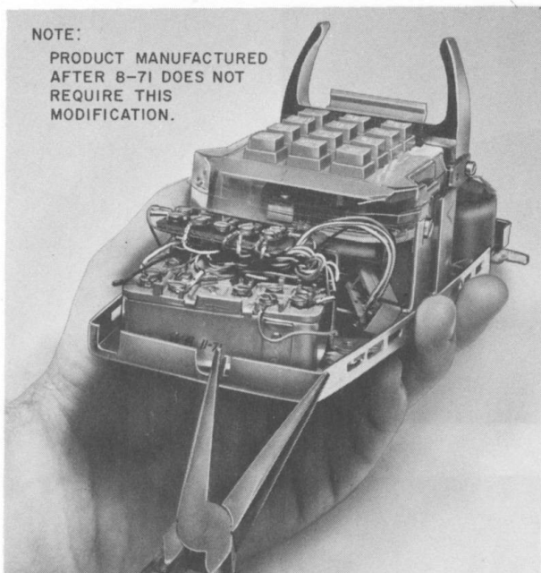
Fig. 44—Modifying 2554B1M Telephone Set Base to Accommodate Handset Cord Jack
