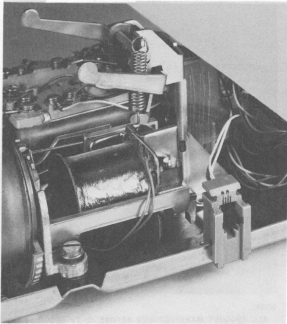
Fig. 37—500D2M or 2500D2M Telephone Set Base With Handset Cord Jack Installed
