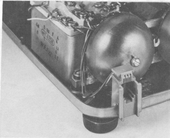
Fig. 38—2500D2M Telephone Set Base With Mounting Cord Jack Installed (500D2M Telephone Set Base is Similar)
