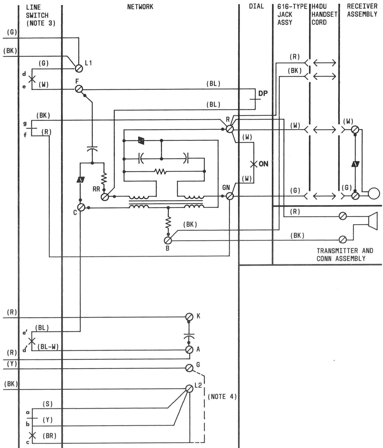
Fig. 3 - CS881C105, CS881C107, or CS881C108 Telephone Set, Connections (Sheet 2 of 2)
