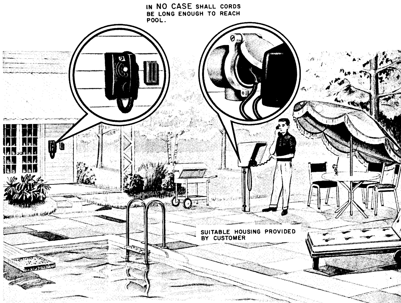
Fig. 1 — Recommended Installation of Pool and Patio Telephone
