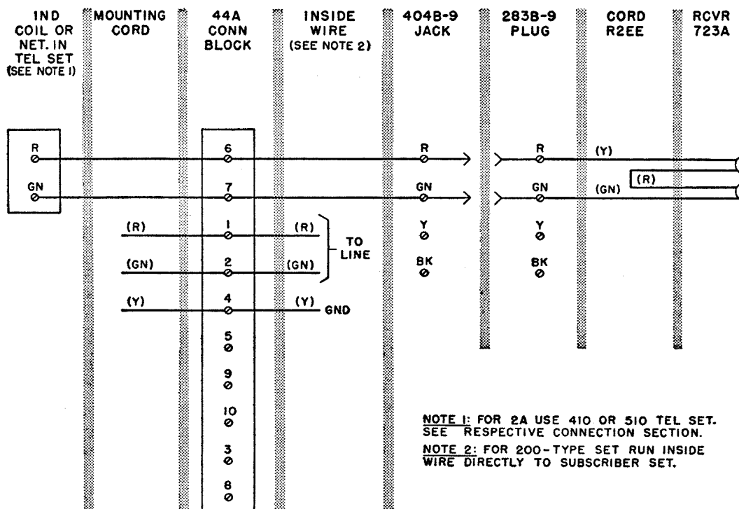
Fig. 1 - 2A, with Key in Set, and 2B Key Equipment Connection Diagram
