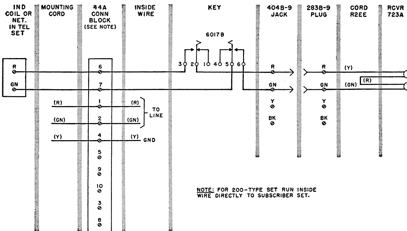
Fig. 2 - 2A Key Equipment with External Key Connection Diagram
