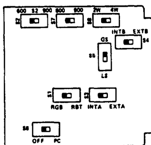
figure 5. Option location
