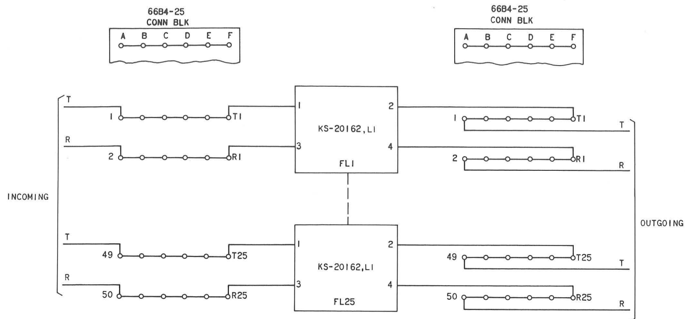
A. KS-20337, LI FILTER, CONNECTIONS
