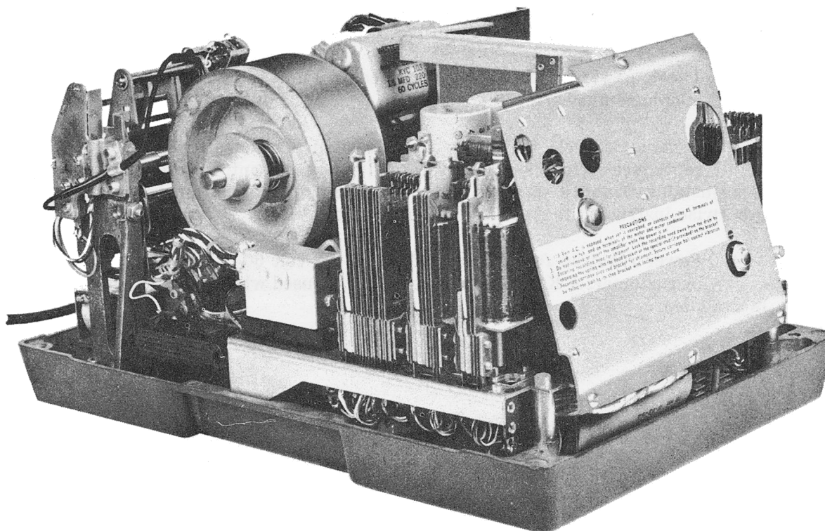
Fig. 2 — 2AB Telephone Answering Set, Cover Removed
