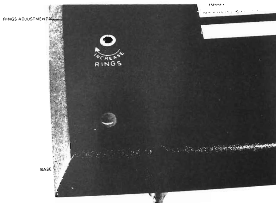
Fig. 2—Rings Adjustment
