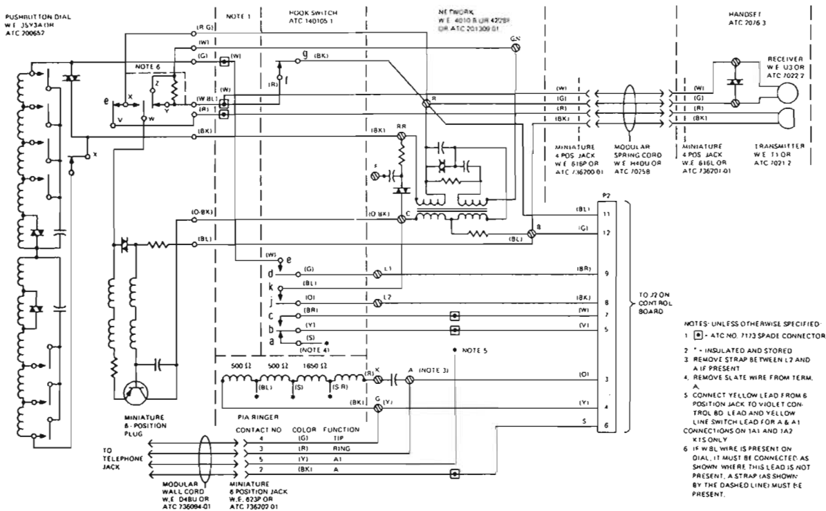
Fig. 6—Model 1000T Connections for Pushbutton Dial
