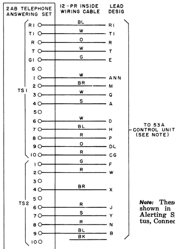
Fig. 1 — Connection Diagram for 2AB Telephone Answering Set
