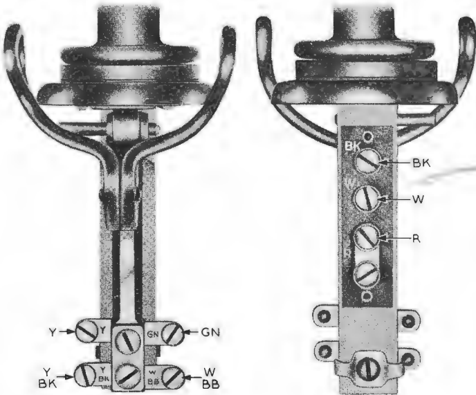
FIG. 3—C1-3 HANDSET MOUNTING
