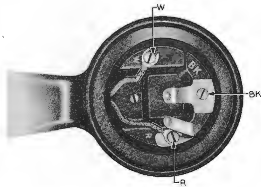
FIG. 2—F1A-3 AND F4 HANDSET
