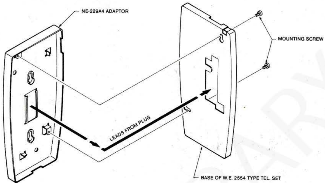
Fig. 20 - NE-229A4 Adaptor
