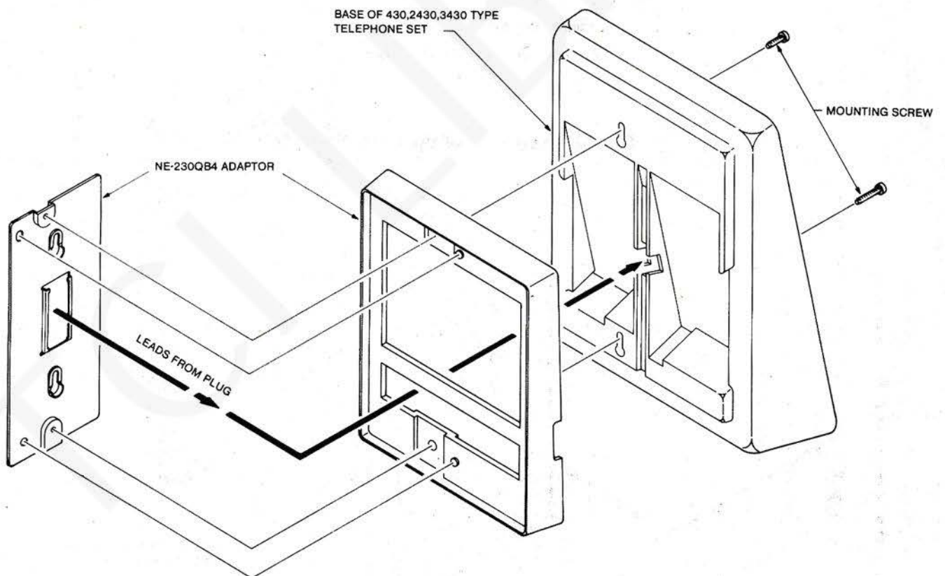
Fig. 21 - NE-230QB4 Adaptor
