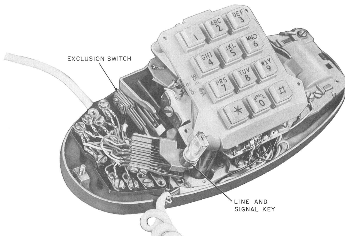
Fig. 2 — 2714A Telephone Set, Interior
