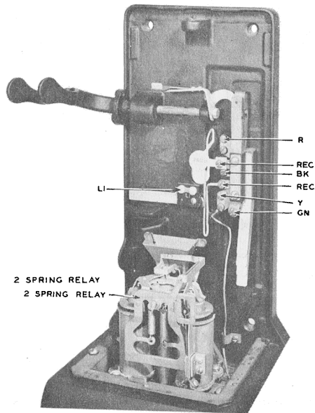
FIG. 3—LOWER HOUSING AND BACKPLATE TERMINALS
