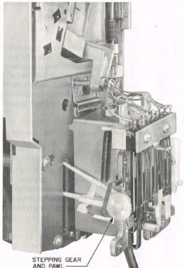
Fig. 3 - Coin Chute and Totalizer, Cover Removed
