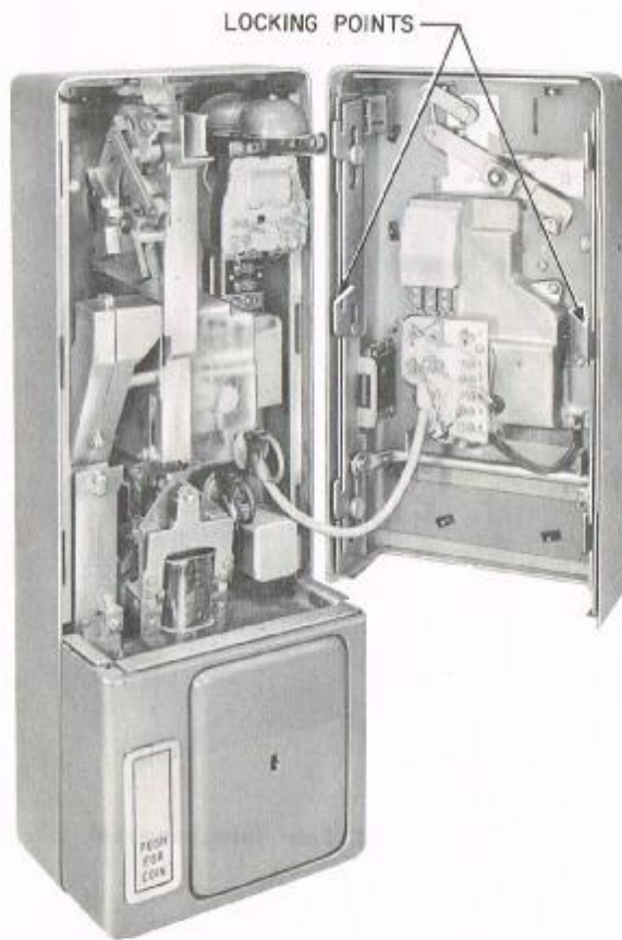
Fig. 2 - 1A1 Coin Telephone Set, Inside View
