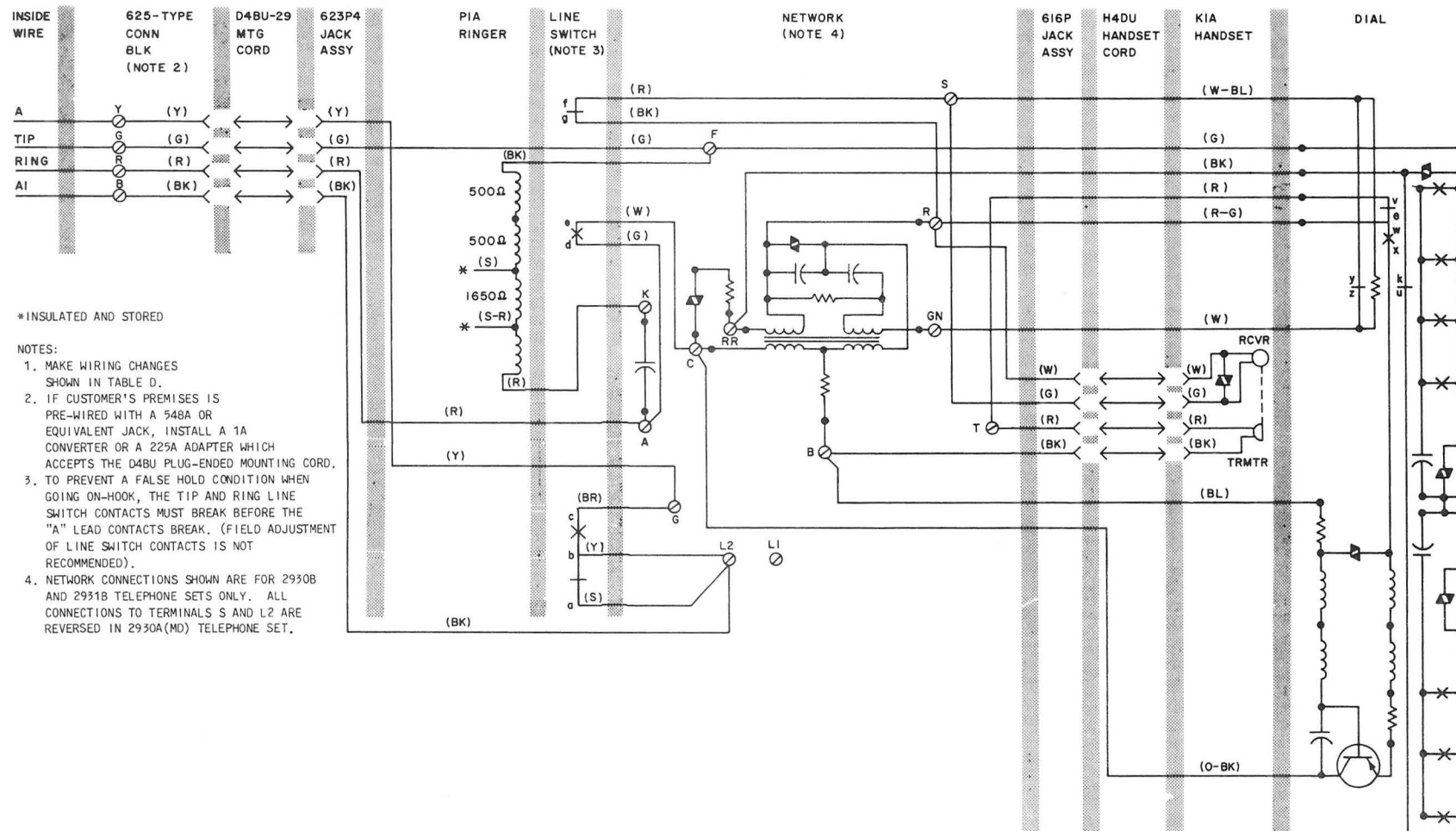
Fig. 11—2930A- (MD), 2930B- (MD), or 2931B-Type (MD) Telephone Set Wired for 1A1 or 1A2 KTS
