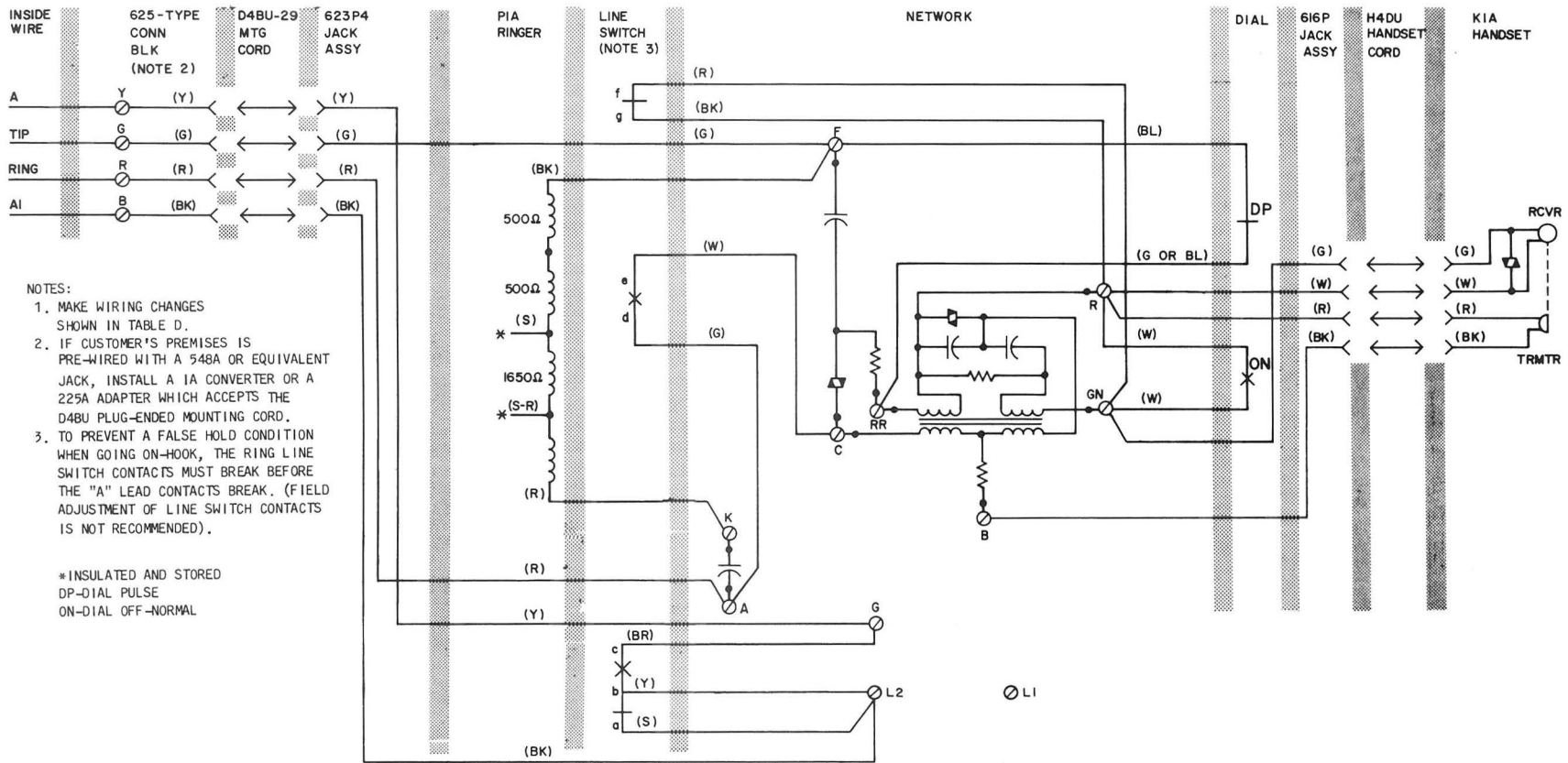
Fig. 10—930A- (MD) or 930B-Type (MD) Telephone Set Wired for 1A1 or 1A2 KTS
