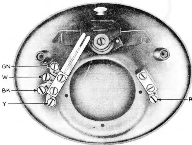
FIG. 5—D1-TYPE HANDSET MOUNTING
