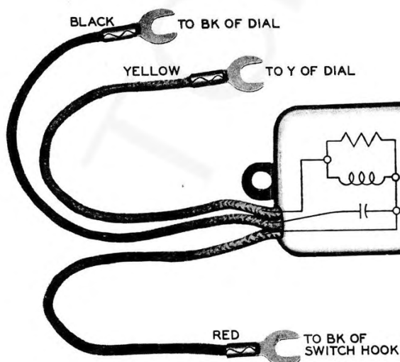
FIG. 6—61N FILTER CONNECTIONS
