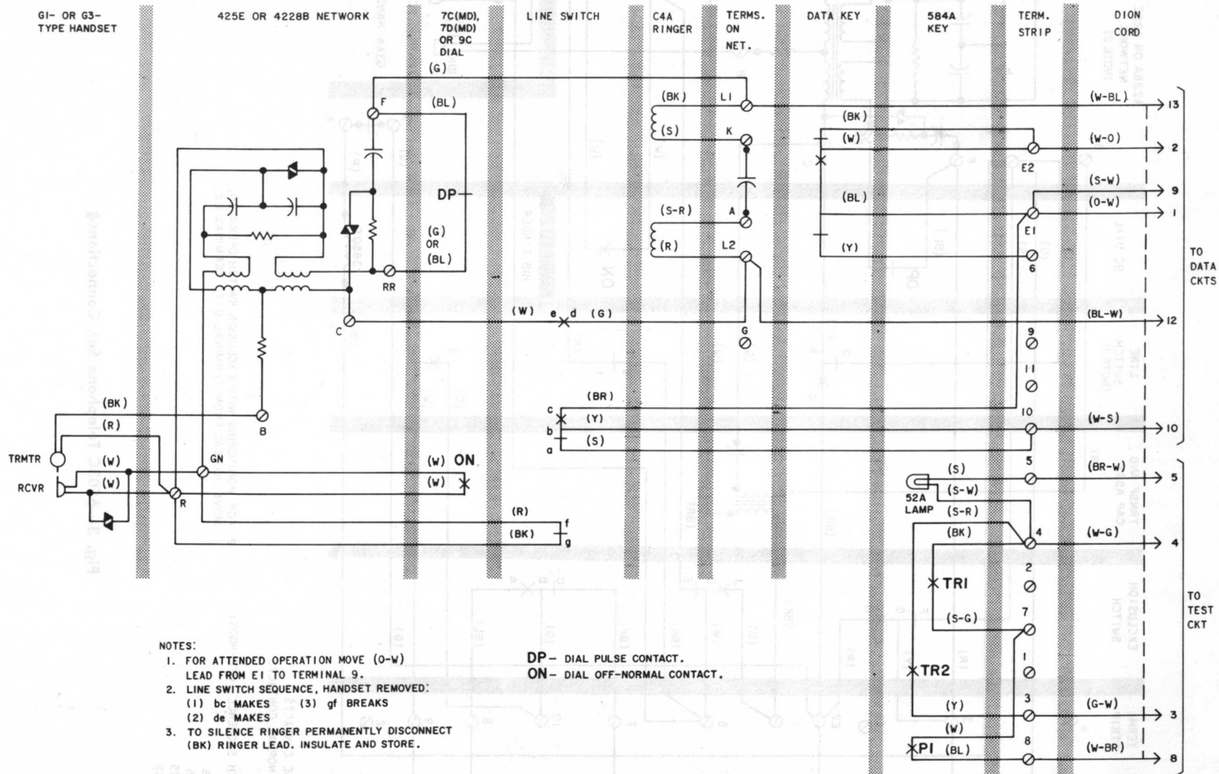
Fig. 4—513B Telephone Set, Connections
