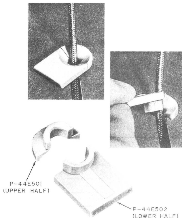
Fig. 1—Removal of Handset Cord Grommet
