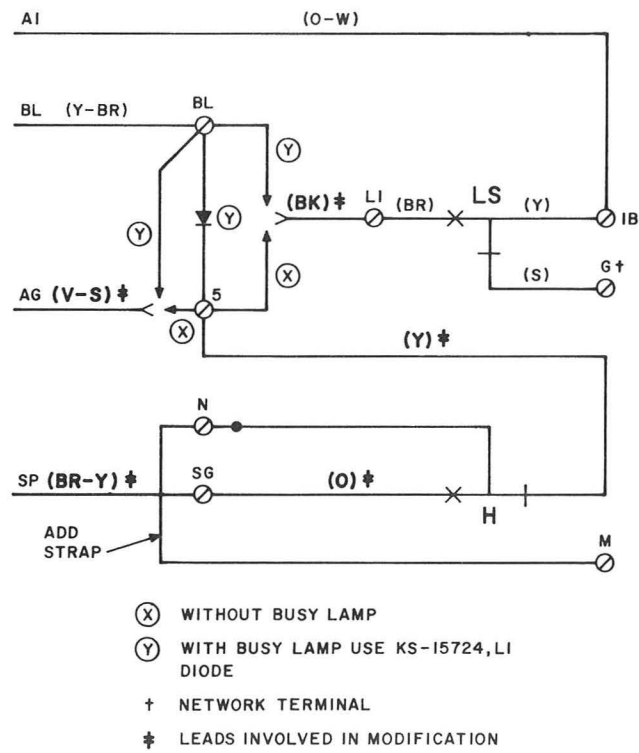
Fig. 4—Set Modified For I Hold
