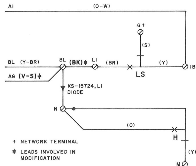
Fig. 3—Station Busy Lamp Circuit, 1A1 or 1A2 KTS
