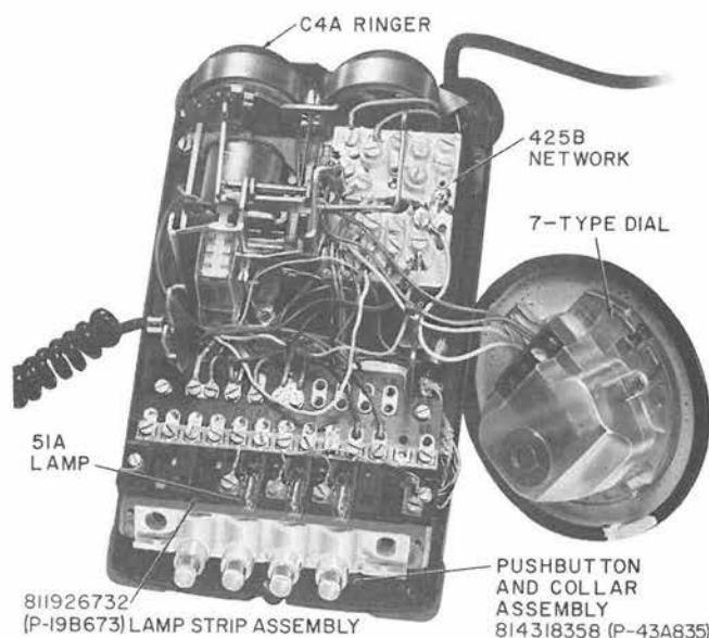
Fig. 2—540-Type Telephone Set, Interior
