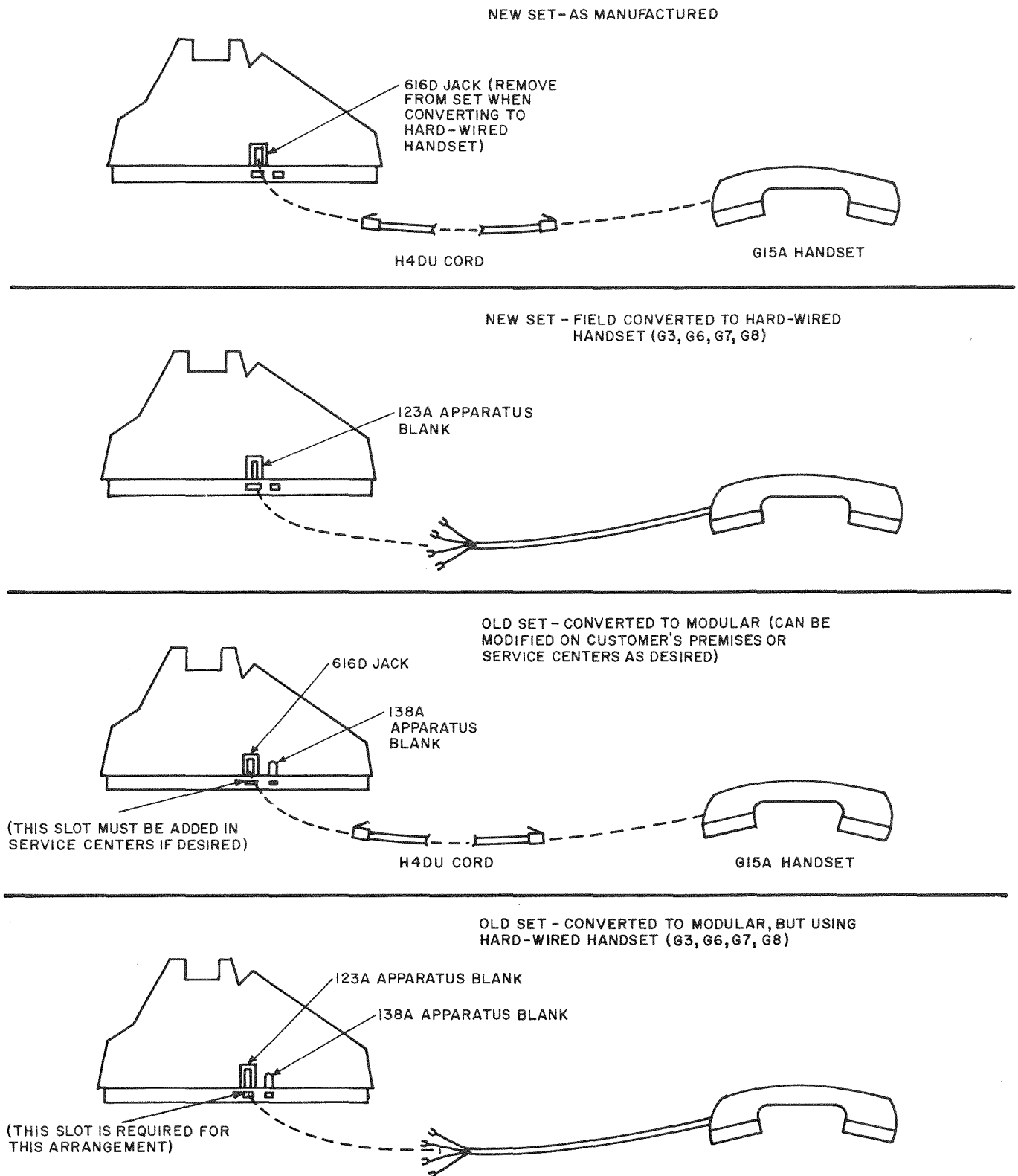
Fig. 5—543DB Key Telephone Set Arranged for Handset Modularity
