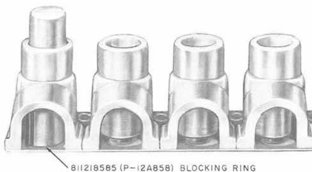
Fig. 4—811218585 (P-12A858) Blocking Ring, Installed
