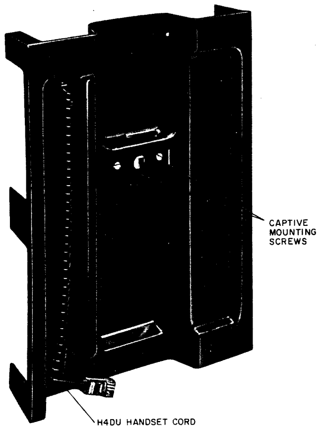
Fig. 2—840399455 Faceplate Assembly
