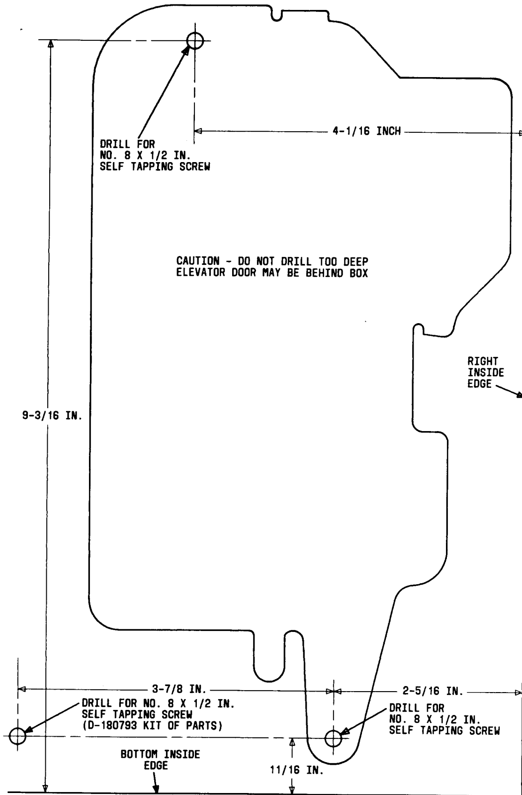
Fig. 6—Outlet Box Mounting Hole Drilling Information
