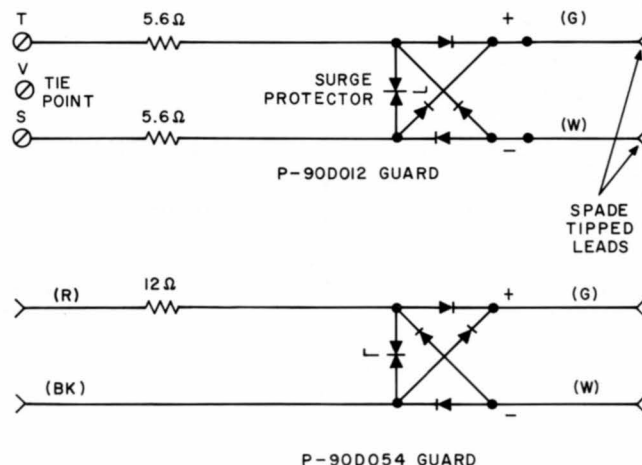
Fig. 2 — Polarity Guards With Surge Protector for TOUCH-TONE Dials
