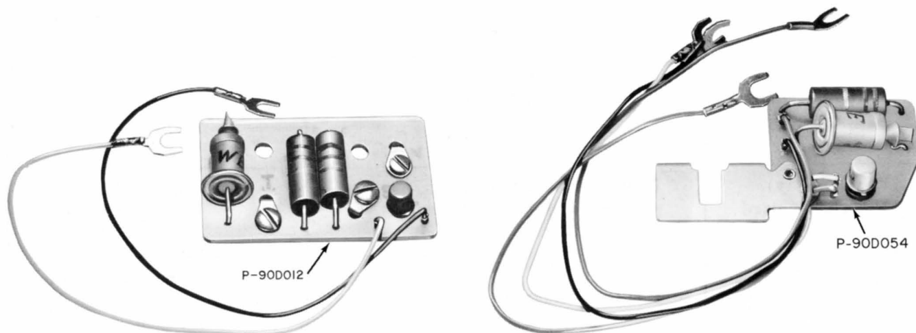
Fig. 1 — Guard Assemblies
