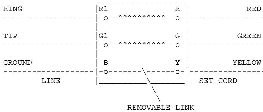
Fig. 4--40BA Capacitor Schematic
