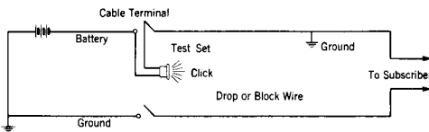
Fig. 3 - Battery Side Grounded
