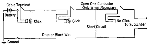
Fig. 7—Tests to Locate Short Circuits
