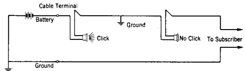
Fig. 4 - Battery Side Grounded
