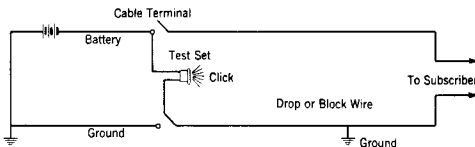
Fig. 2 - Ground Side Grounded
