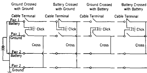
Fig. 8 — Tests to Locate Crosses
