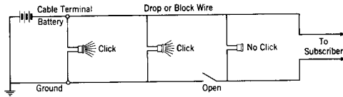
Fig. 6 — Test for Locating an Open
