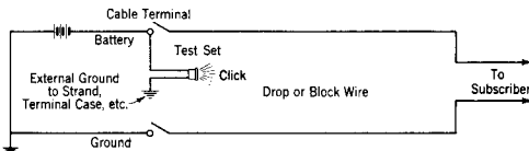
Fig. 1 - Test to Determine Battery Side of Line
