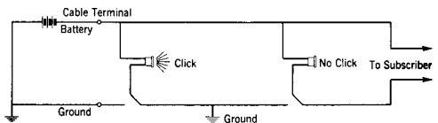
Fig. 5 - Ground Side Grounded
