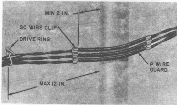
Fig. 6—Block Wires Crossing Over Pipe
