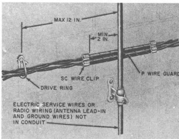
Fig. 12—Block Wire Crossing Behind Foreign Wire
