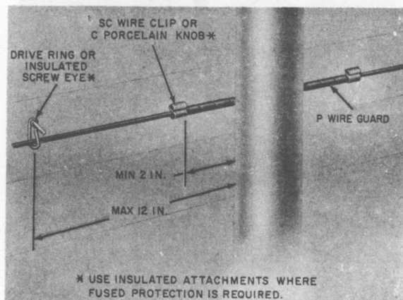
Fig. 10—Drop Wire Crossing Behind Pipe
