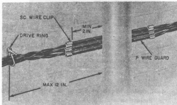
Fig. 7—Block Wires Crossing Behind Pipe
