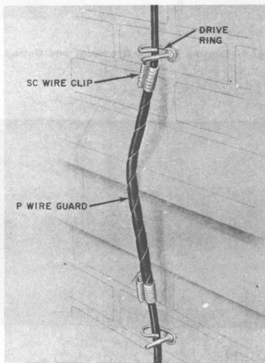
Fig. 3—Crossing Masonry Building Projection
