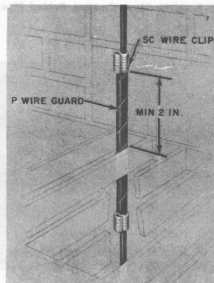
Fig. 5—Protecting Wire Run Through Stationary Metal Grating
