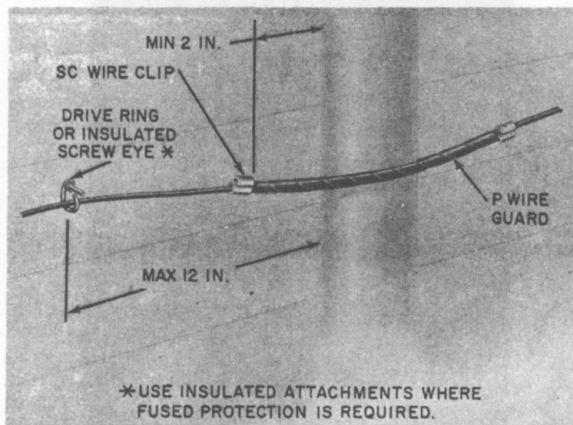
Fig. 8—Drop Wire Over Pipe
