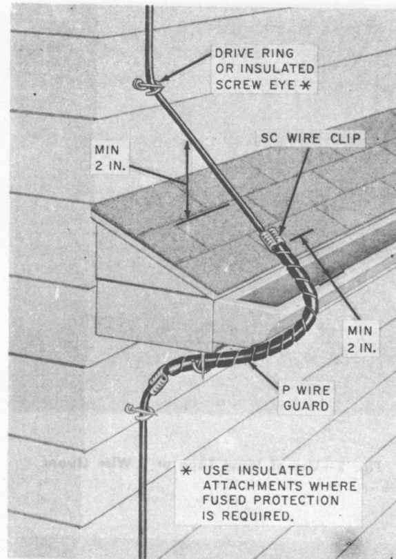
Fig. 9—Crossing Building Overhangs and Gutters
