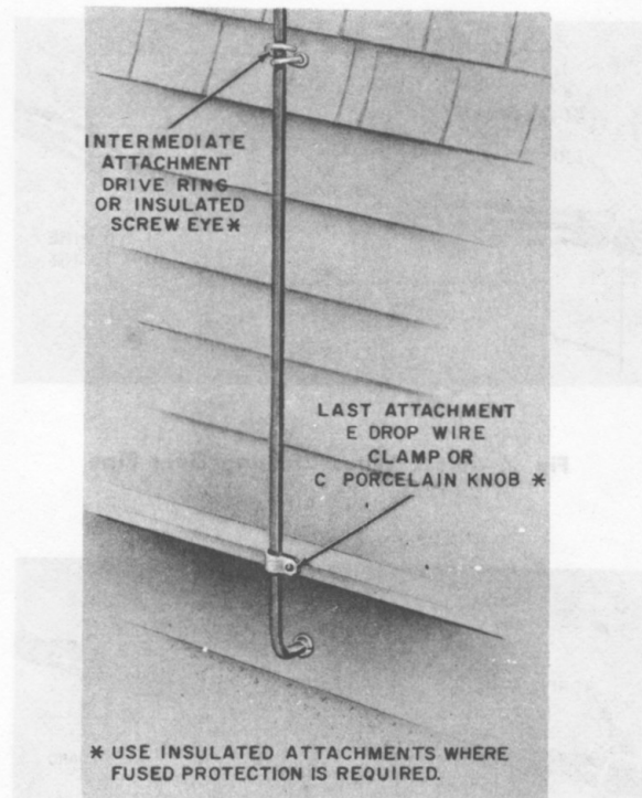
Fig. 4—Crossing Wood or Stucco on Wood Building Projection
