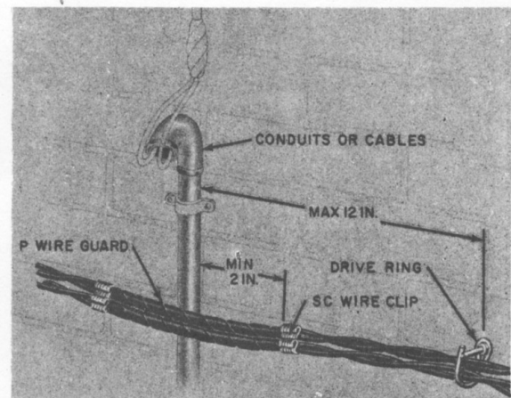
Fig. 14—Block Wire Crossing Over Conduit
