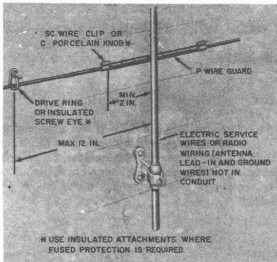
Fig. 11—Drop Wire Crossing Behind Foreign Wire
