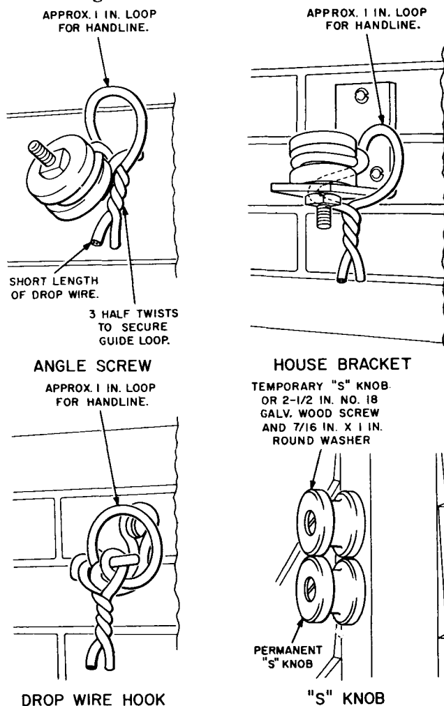
Fig. 9 — Temporary Guide Loop
