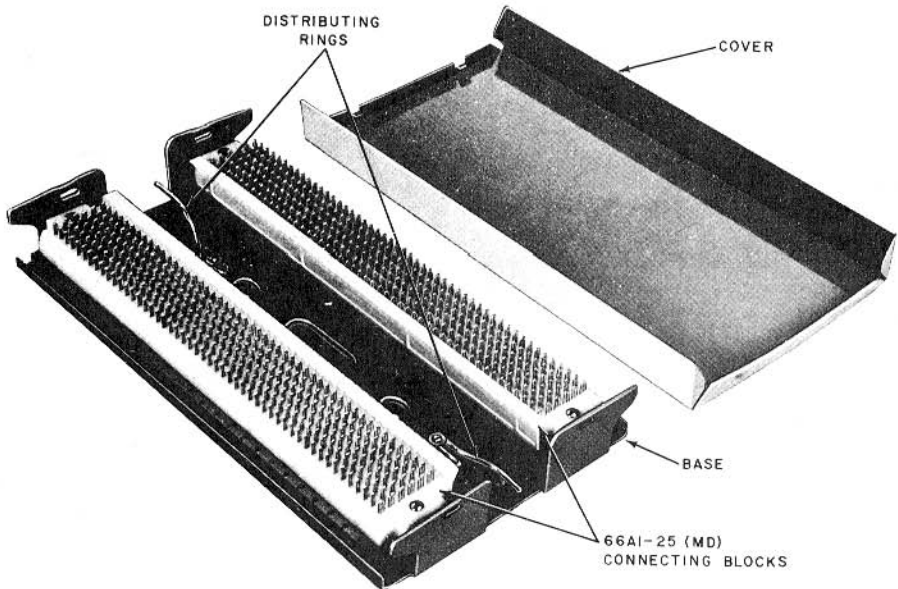
Fig. 11—66A1-25 (MD) Connecting Block
