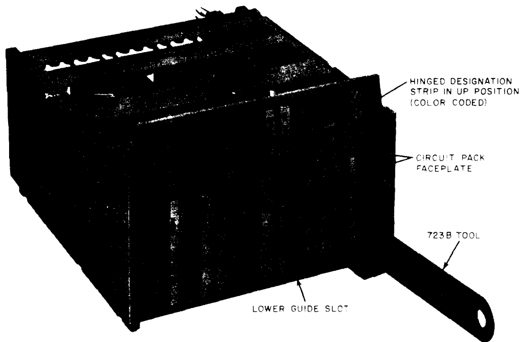
Fig. 5—Apparatus Mounting With Hinged Designation Strip in Raised Position
