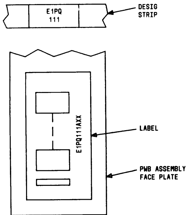
Fig. 7—Typical Bar Code Label and Designation Strip
