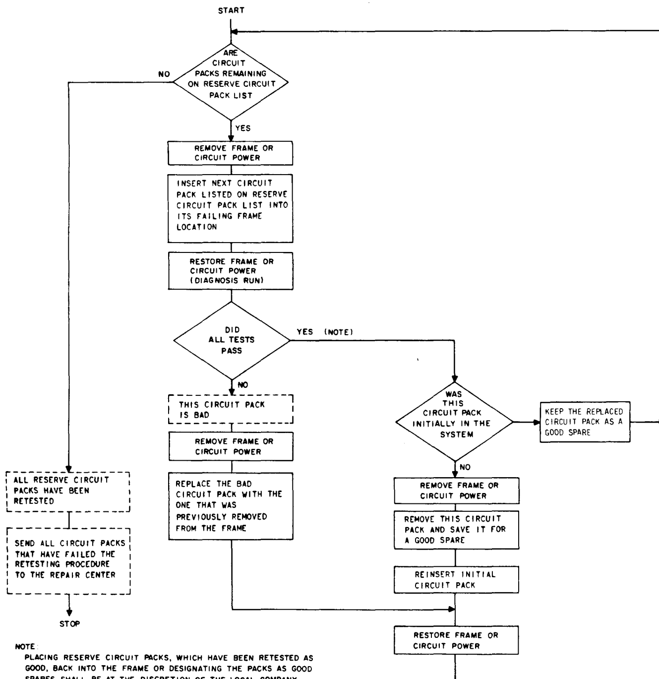
Fig. 13—Procedure for Retesting Reserve Circuit Packs
