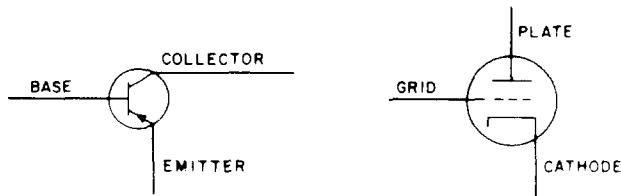
Fig. 1—Comparison of Transistor and Vacuum Tube
