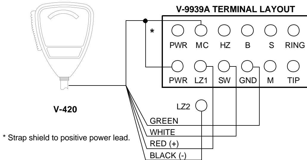
FIGURE 1. CONNECTING ARRANGEMENT
