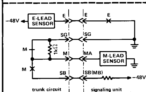
figure 7c. Type III E&M signaling interface
