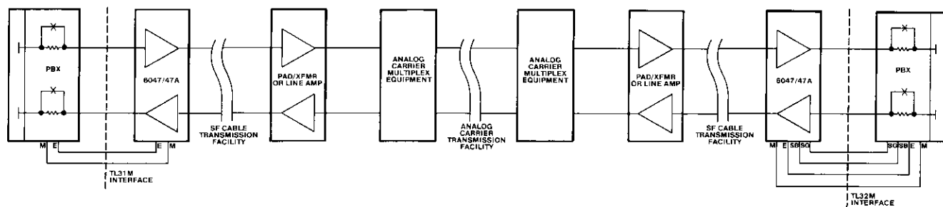
figure 3. Typical long-haul analog tie-trunk circuit using 6047 or 6047A
