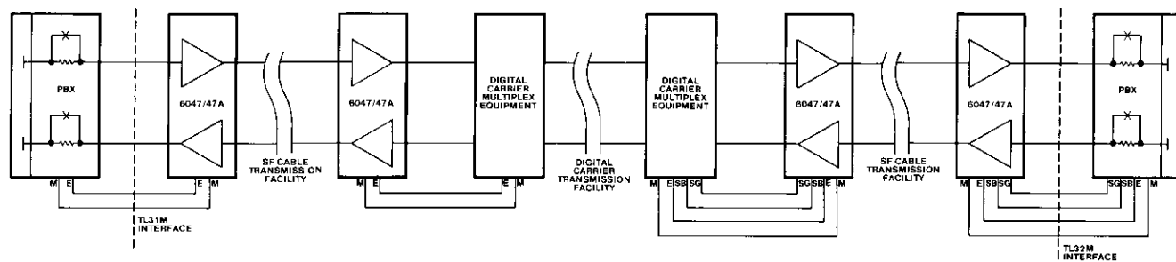
figure 4. Typical long-haul digital tie-trunk circuit using 6047 or 6047A
