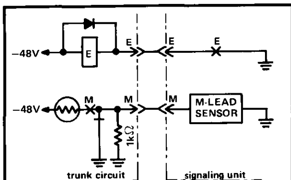
figure 7a. Type I E&M signaling interface
