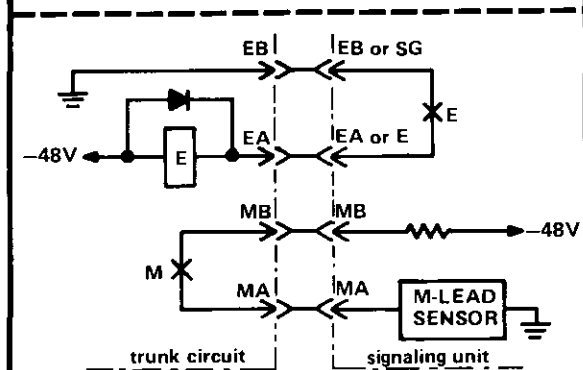
figure 7b. Type II E&M signaling interface
